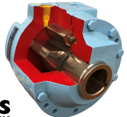
MICROMATIC ROTAC ® ROTARY VANE ACTUATOR
